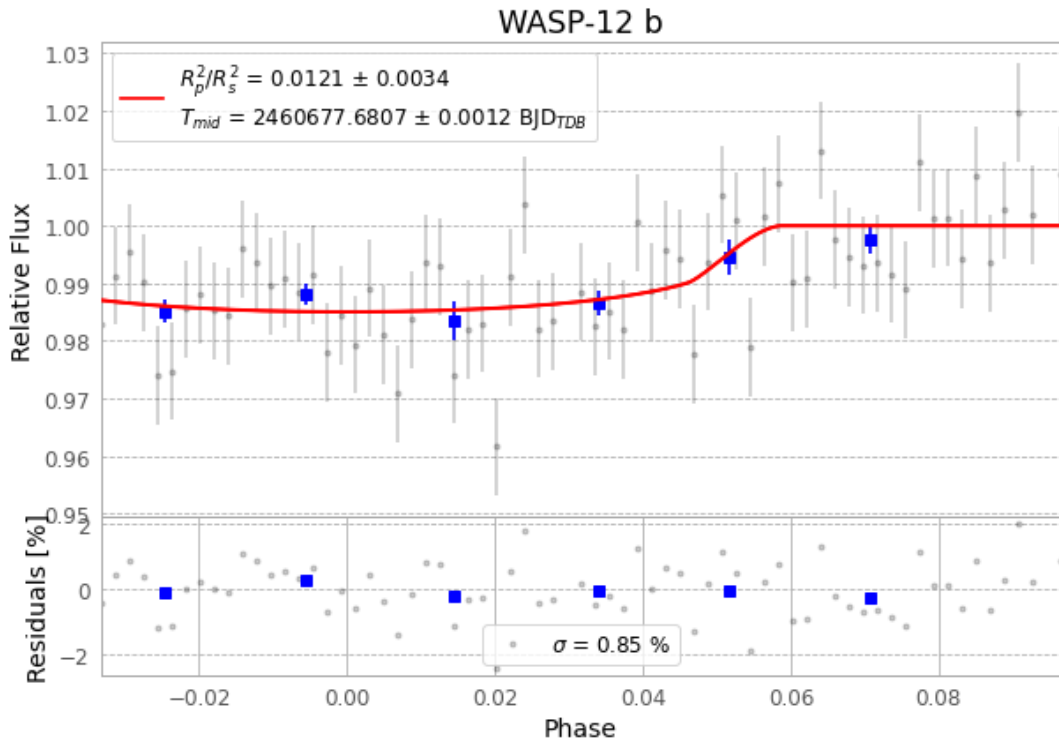
Figure 1 — FinalLightCurve_WASP-12 b_2025-01-01.png (SHA-256 3f2dc8c25fe80b72...)
