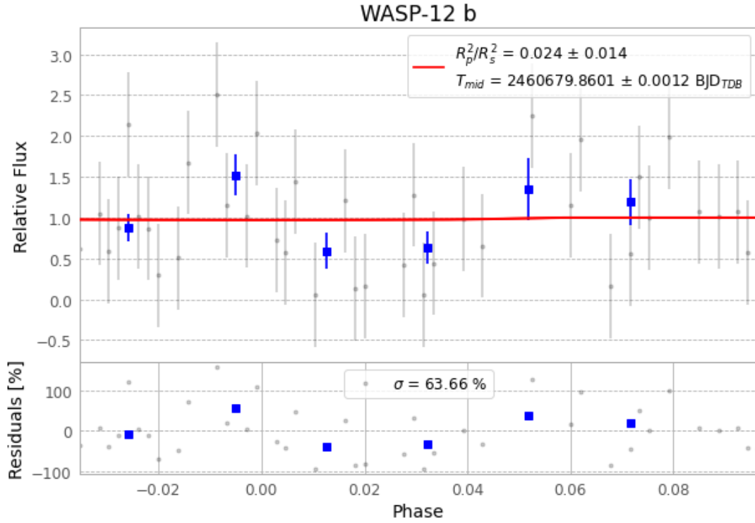
Figure 1 — FinalLightCurve_WASP-12 b_2025-01-04.png (SHA-256 7a5a77bbf2a274d9...)
