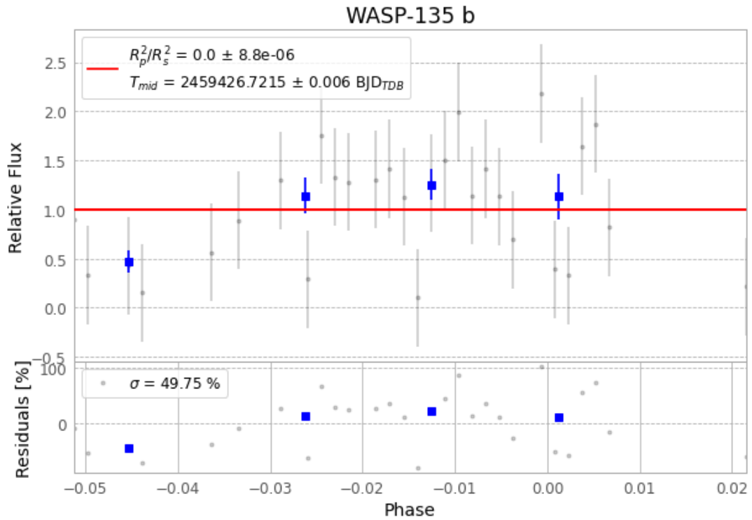
Figure 1 — FinalLightCurve_WASP-135 b_2021-07-30.png (SHA-256 ad686f3a9800cb74...)
