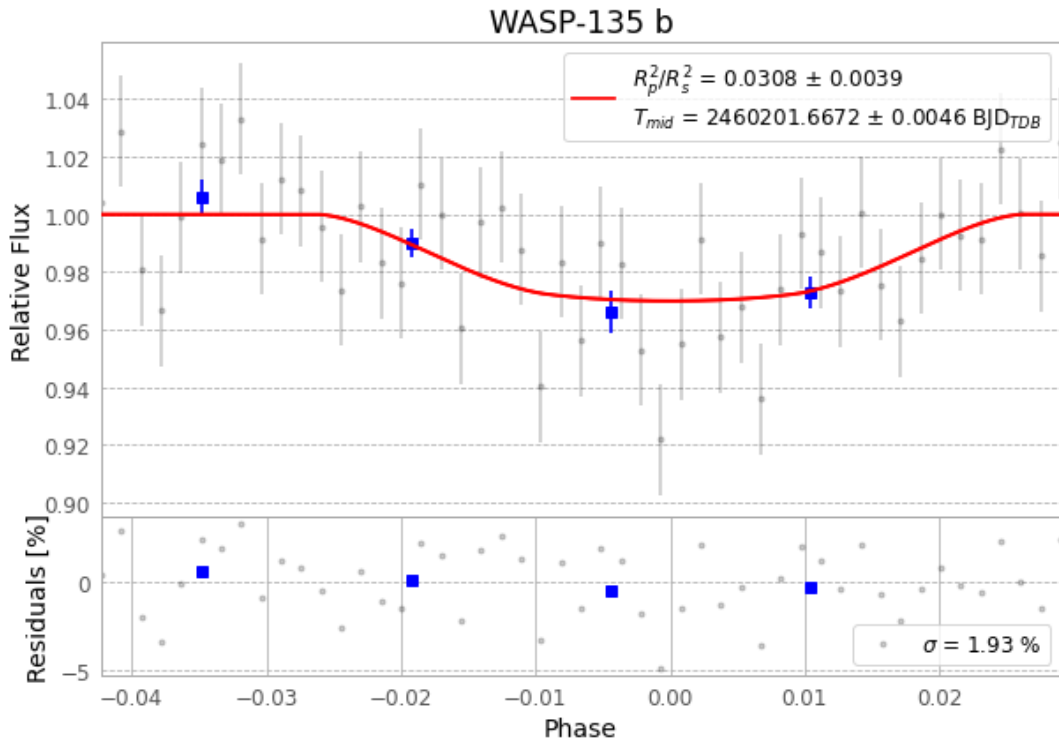
Figure 1 — FinalLightCurve_WASP-135 b_2023-09-13.png (SHA-256 484579a128cb7bed...)
