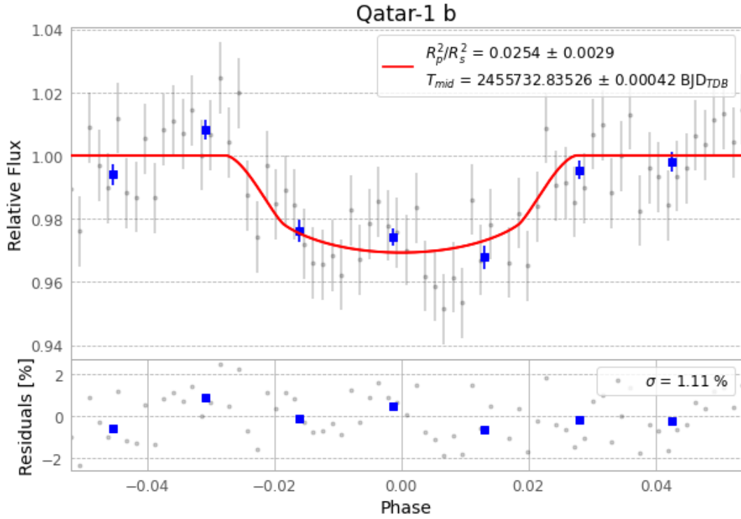
Figure 1 — FinalLightCurve_Qatar-1 b_2011-06-19.png (SHA-256 27e5c4b586489f43...)
