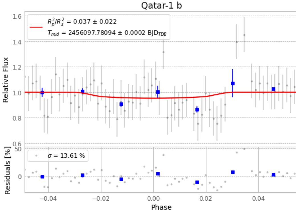
Figure 1 — FinalLightCurve_Qatar-1 b_2012-06-18.png (SHA-256 c8c2197cf931e98c...)
