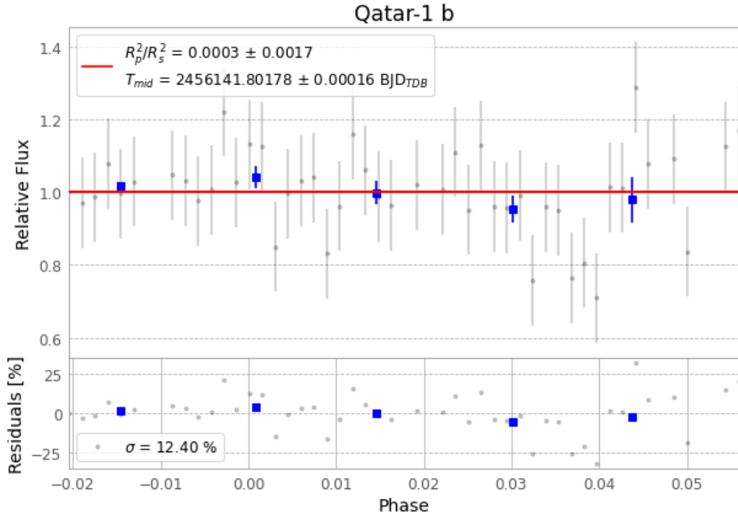
Figure 1 — FinalLightCurve_Qatar-1 b_2012-08-01.png (SHA-256 b7a4027cc8cb7b18...)
