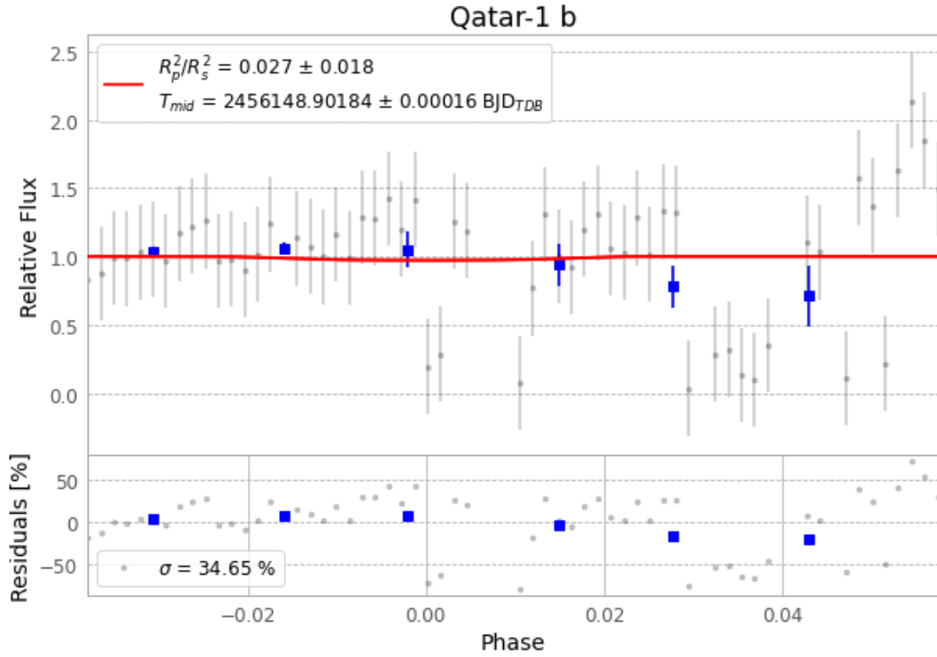
Figure 1 — FinalLightCurve_Qatar-1 b_2012-08-09.png (SHA-256 a7c5a08cdca4d62e...)
