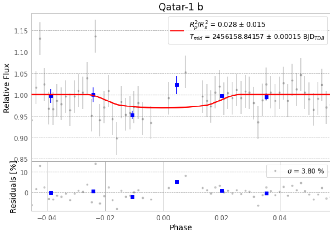
Figure 1 — FinalLightCurve_Qatar-1 b_2012-08-18.png (SHA-256 799c88ecf8a5de73...)
