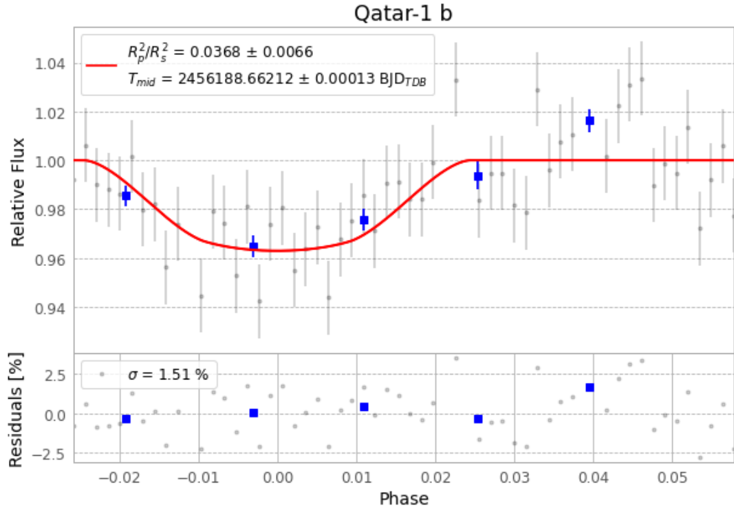
Figure 1 — FinalLightCurve_Qatar-1 b_2012-09-17.png (SHA-256 deb86f42d04acc9c...)
