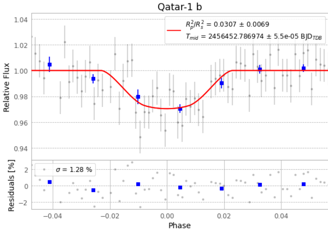
Figure 1 — FinalLightCurve_Qatar-1 b_2013-06-08.png (SHA-256 24bbffbf033e991...)
