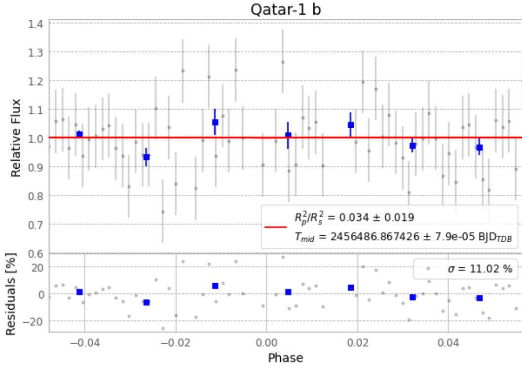
Figure 1 — FinalLightCurve_Qatar-1 b_2013-07-13.png (SHA-256 202a782de1a09b82...)
