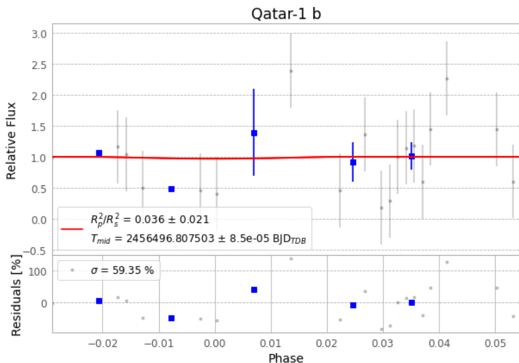
Figure 1 — FinalLightCurve_Qatar-1 b_2013-07-22.png (SHA-256 8ca8d5bb16e0e675...)
