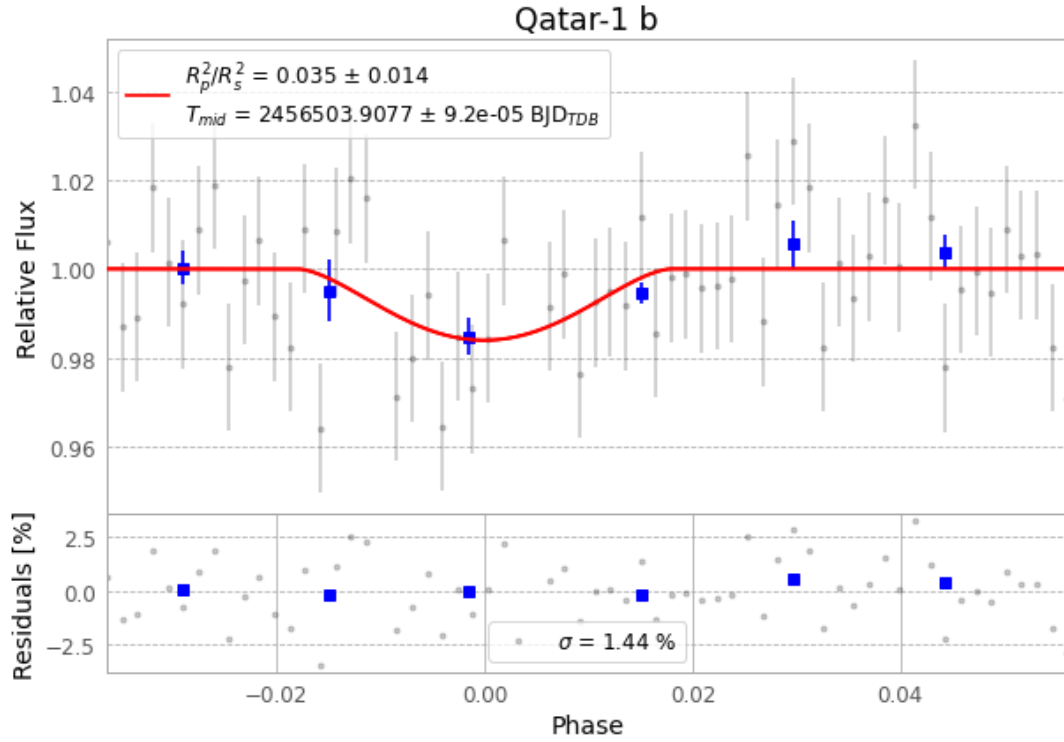
Figure 1 — FinalLightCurve_Qatar-1 b_2013-07-30.png (SHA-256 d7c5a1ffcd7f2a40...)
