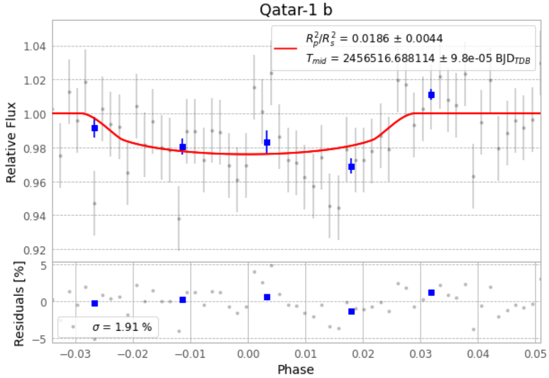
Figure 1 — FinalLightCurve_Qatar-1 b_2013-08-11.png (SHA-256 d0cbd3fe43165e0e...)
