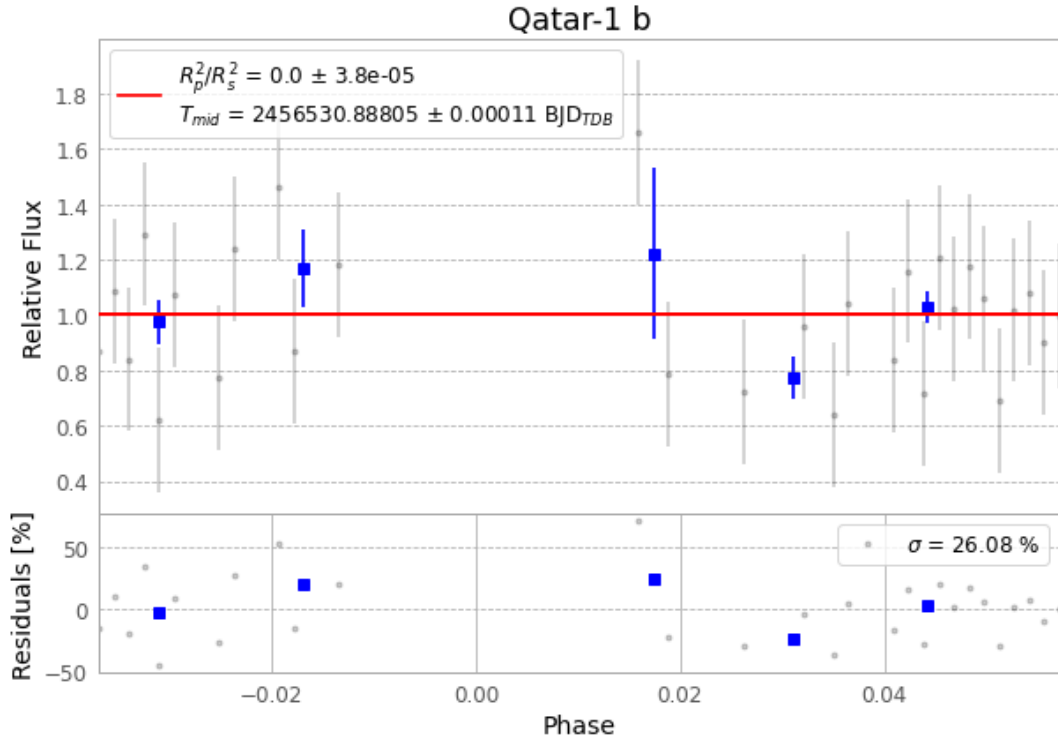
Figure 1 — FinalLightCurve_Qatar-1 b_2013-08-26.png (SHA-256 6c439a044100bcc9...)
