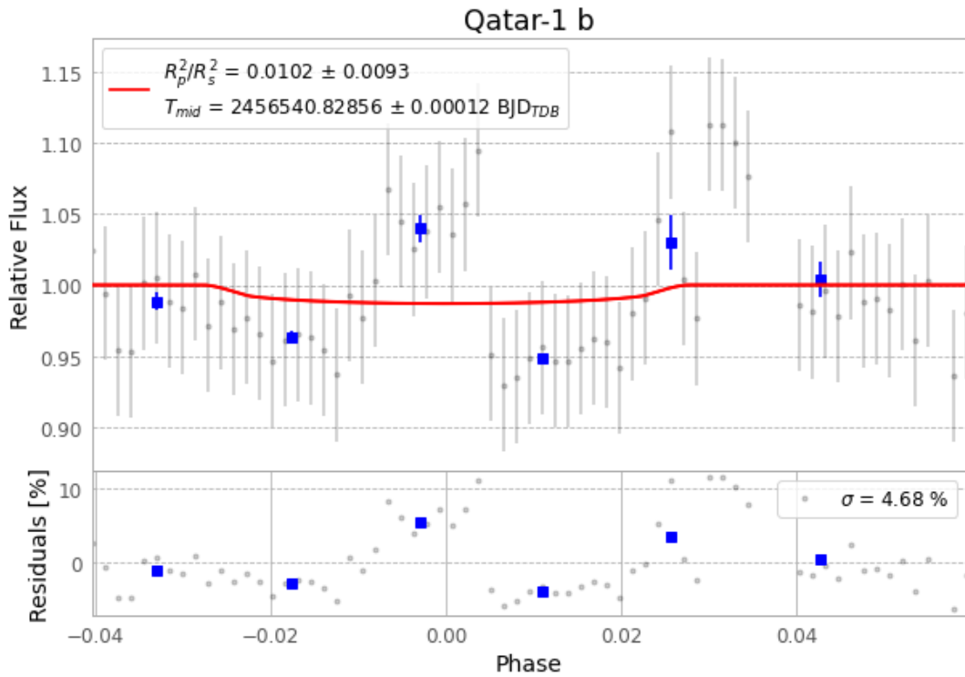
Figure 1 — FinalLightCurve_Qatar-1 b_2013-09-04.png (SHA-256 1ab1dde7100deadc...)
