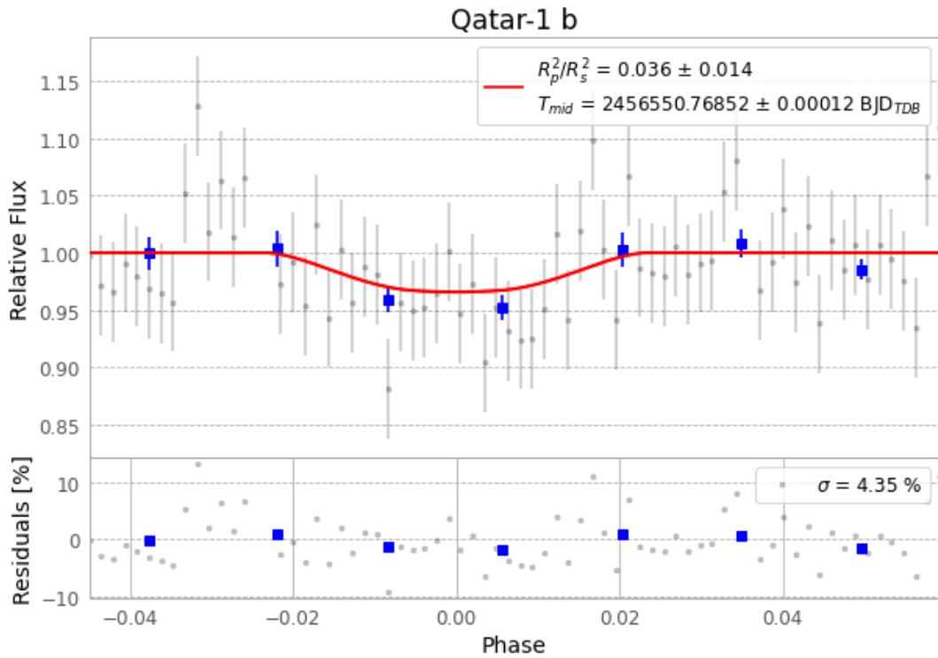
Figure 1 — FinalLightCurve_Qatar-1 b_2013-09-14.png (SHA-256 655f6111e5c39b62...)
