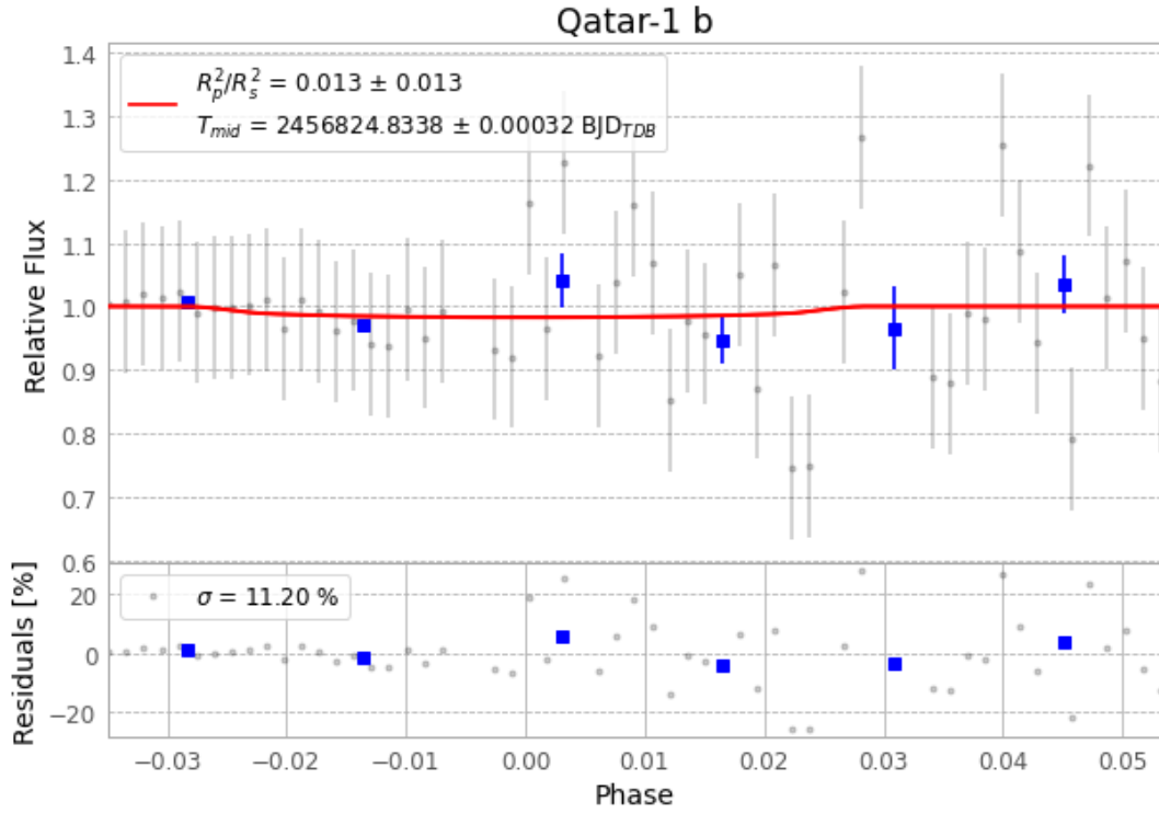
Figure 1 — FinalLightCurve_Qatar-1 b_2014-06-15.png (SHA-256 80e2db250b11578a...)
