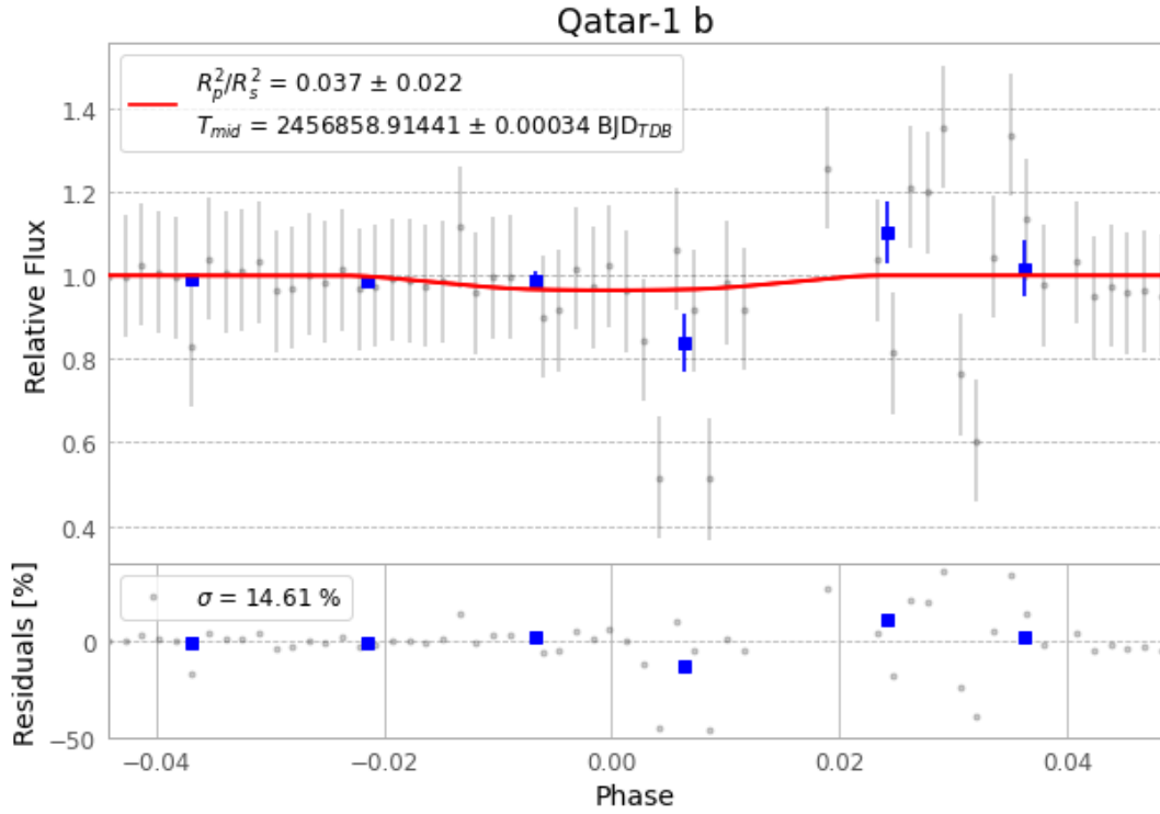
Figure 1 — FinalLightCurve_Qatar-1 b_2014-07-20.png (SHA-256 5f9bcef07655b0f5...)
