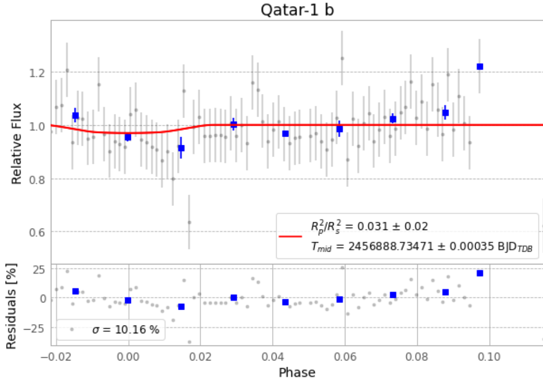
Figure 1 — FinalLightCurve_Qatar-1 b_2014-08-18.png (SHA-256 a740ffe088ea298c...)
