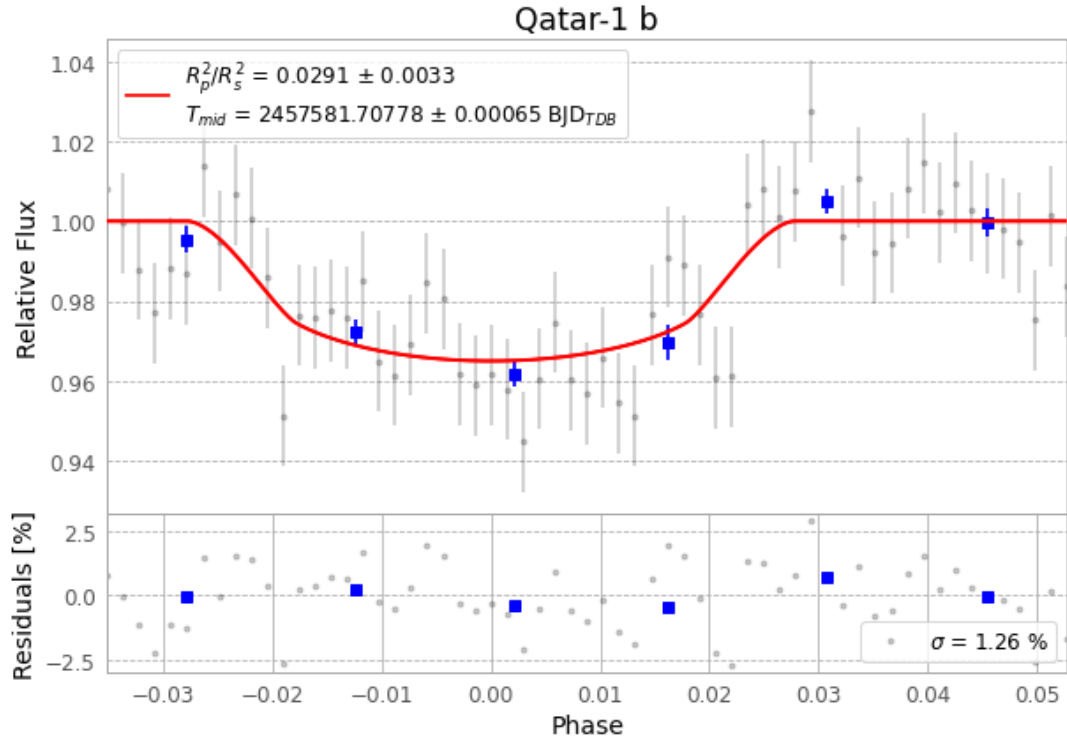
Figure 1 — FinalLightCurve_Qatar-1 b_2016-07-11.png (SHA-256 5b47b5b6586d4bd2...)
