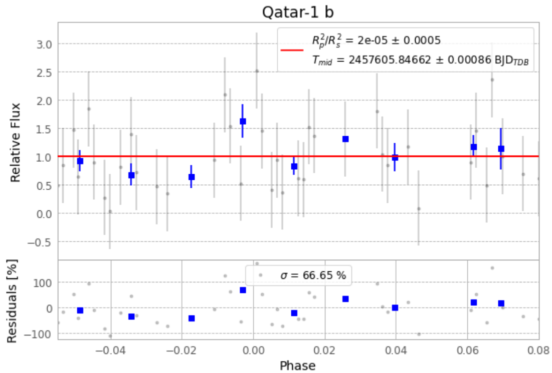
Figure 1 — FinalLightCurve_Qatar-1 b_2016-08-04.png (SHA-256 f91caeacd0c0e54f...)
