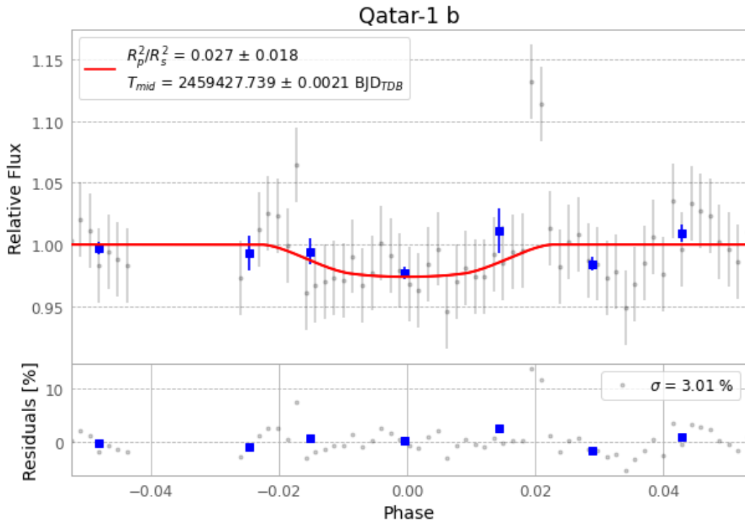
Figure 1 — FinalLightCurve_Qatar-1 b_2021-07-31.png (SHA-256 52f9c596193c2488...)
