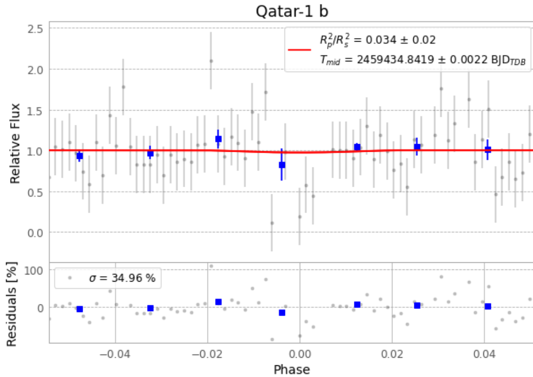
Figure 1 — FinalLightCurve_Qatar-1 b_2021-08-07.png (SHA-256 91f221255997d8f5...)
