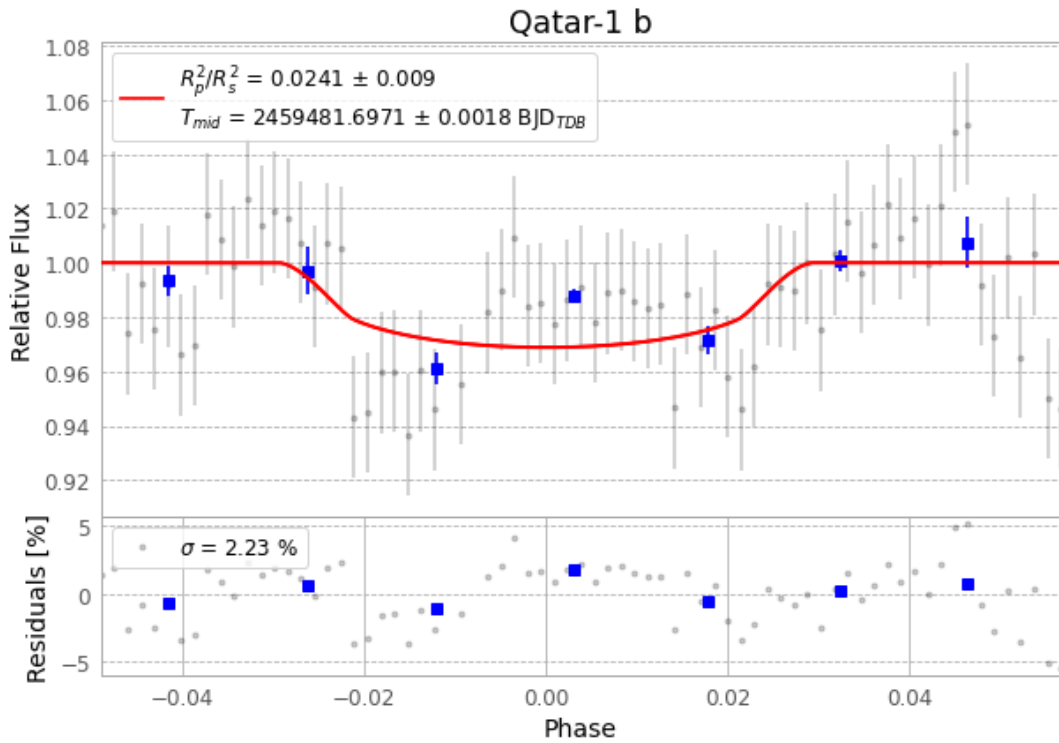
Figure 1 — FinalLightCurve_Qatar-1 b_2021-09-23.png (SHA-256 f62258856cd7c952...)
