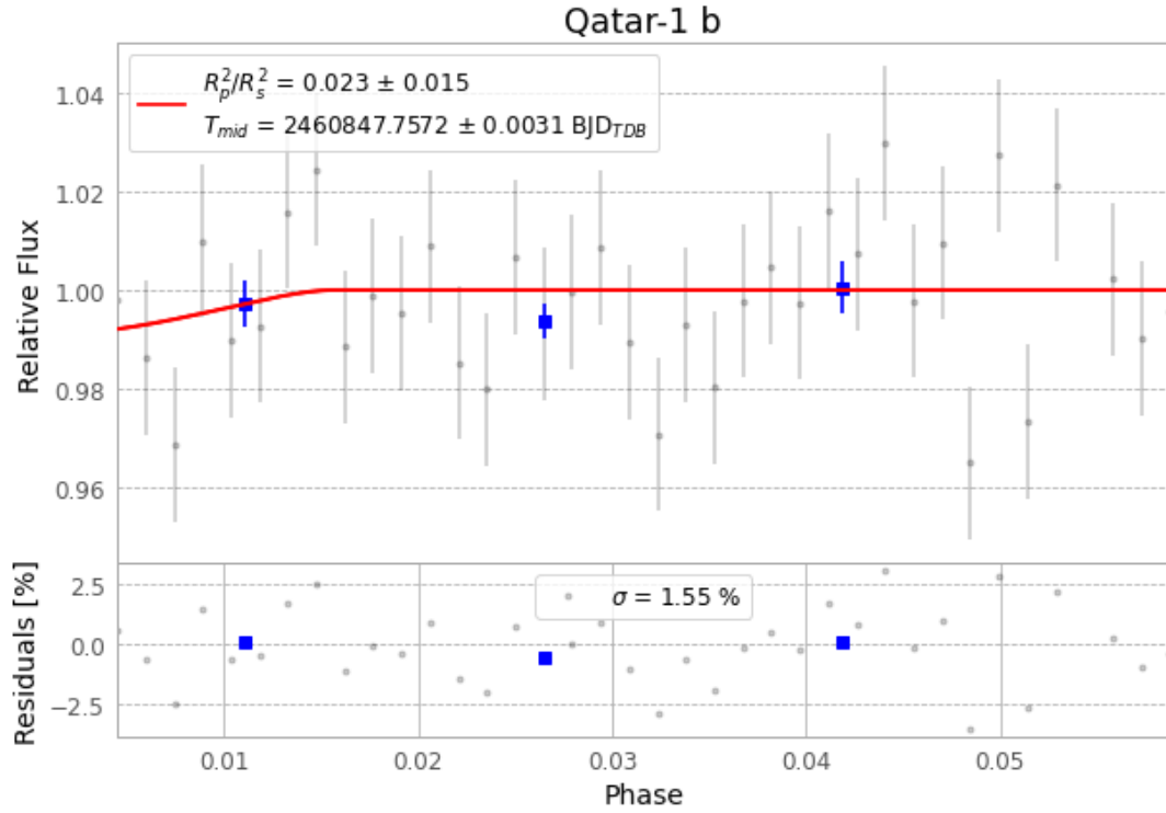
Figure 1 — FinalLightCurve_Qatar-1 b_2025-06-20.png (SHA-256 40cad9912ec1097c...)
