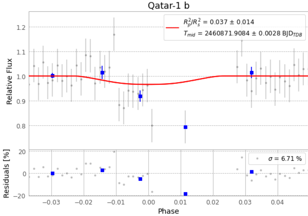
Figure 1 — FinalLightCurve_Qatar-1 b_2025-07-15.png (SHA-256 70076b441f4b3543...)
