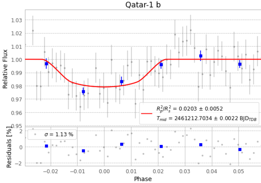
Figure 1 — FinalLightCurve_Qatar-1 b_2026-06-20.png (SHA-256 fea1f4add76daafc...)
