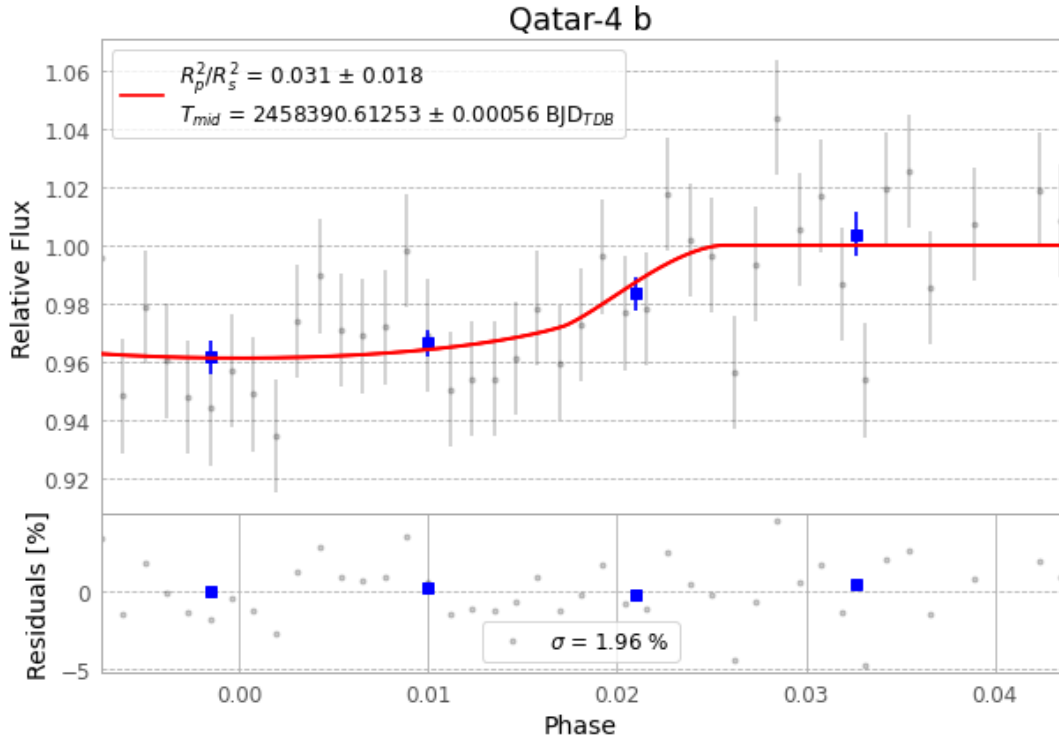
Figure 1 — FinalLightCurve_Qatar-4 b_2018-09-28.png (SHA-256 9f97542c49e680db...)
