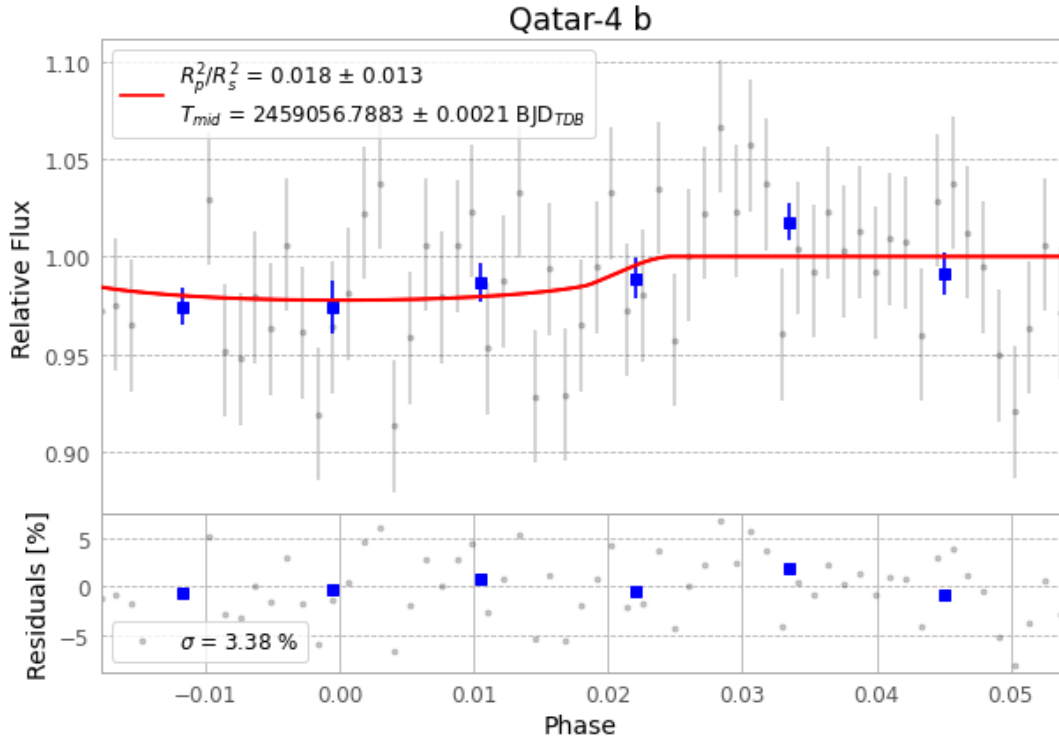
Figure 1 — FinalLightCurve_Qatar-4 b_2020-07-25.png (SHA-256 08c195220880bfa9...)
