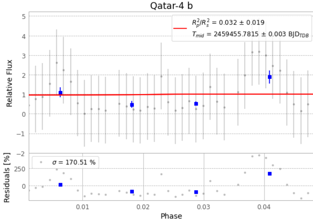
Figure 1 — FinalLightCurve_Qatar-4 b_2021-08-28.png (SHA-256 39a5e5aa33b474ae...)
