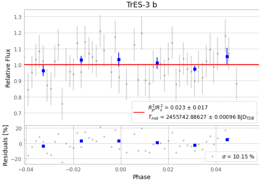
Figure 1 — FinalLightCurve_TrES-3 b_2011-06-30.png (SHA-256 0db71780b5e23c2a...)
