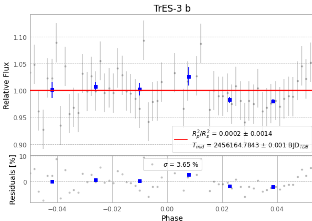
Figure 1 — FinalLightCurve_TrES-3 b_2012-08-24.png (SHA-256 2b521bc5de8967a1...)
