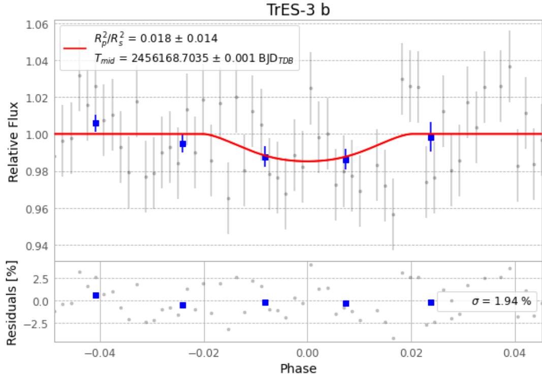
Figure 1 — FinalLightCurve_TrES-3 b_2012-08-28.png (SHA-256 a200077fe1ffdab9...)
