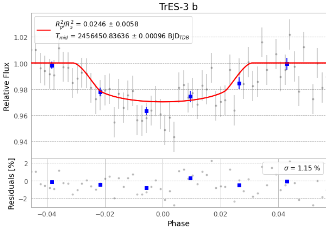
Figure 1 — FinalLightCurve_TrES-3 b_2013-06-06.png (SHA-256 d371fcf58d4a79c9...)
