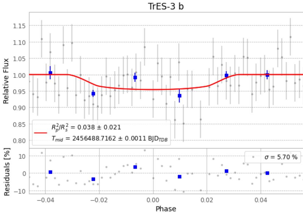
Figure 1 — FinalLightCurve_TrES-3 b_2013-07-14.png (SHA-256 49f70d8433d4f072...)
