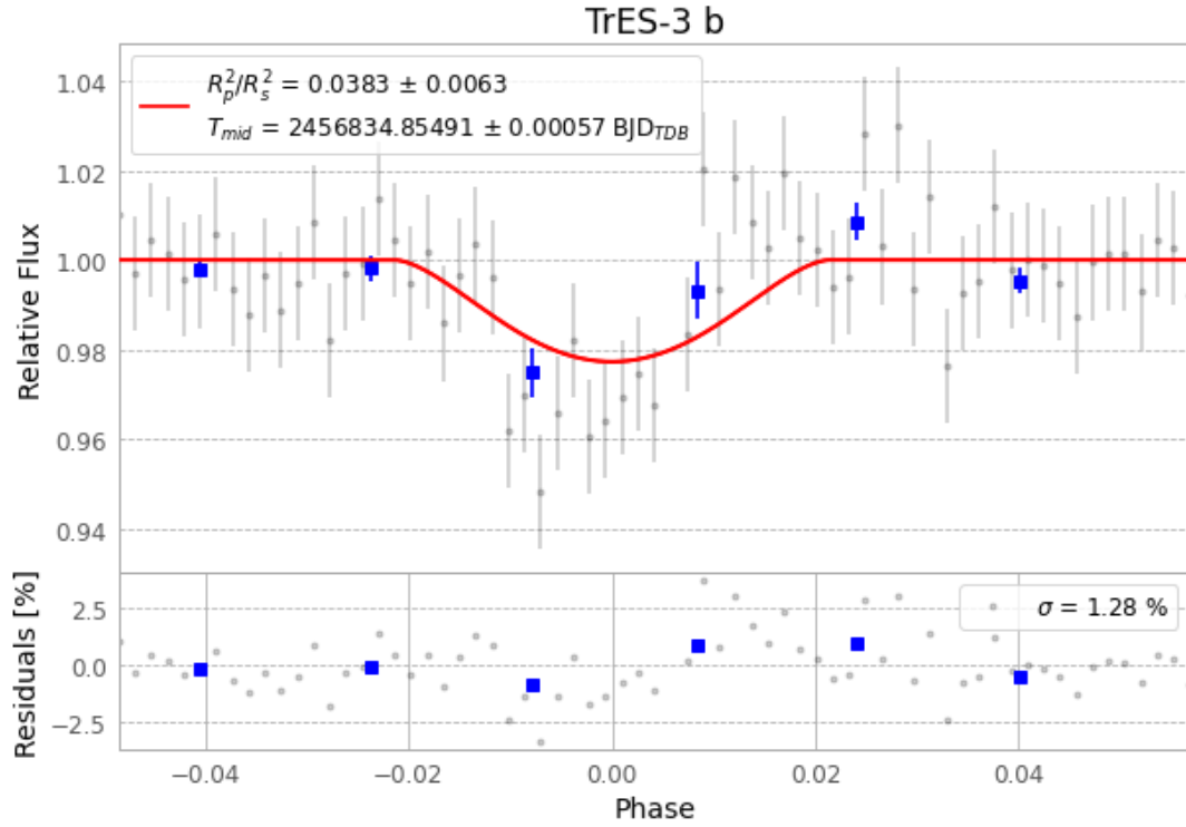
Figure 1 — FinalLightCurve_TrES-3 b_2014-06-25.png (SHA-256 7cdb1c21a41f2243...)
