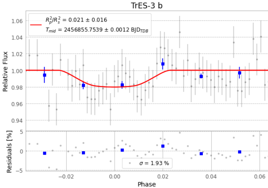
Figure 1 — FinalLightCurve_TrES-3 b_2014-07-16.png (SHA-256 190f1f014a094f3e...)
