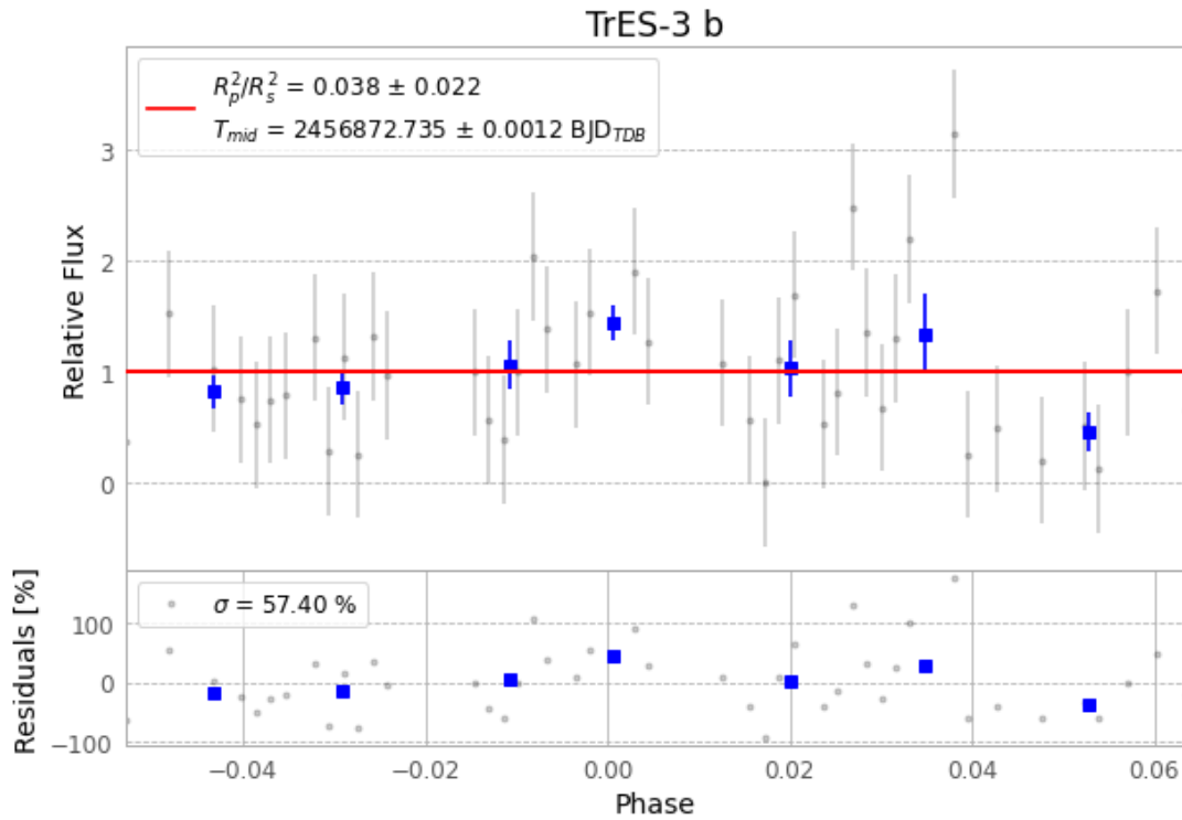
Figure 1 — FinalLightCurve_TrES-3 b_2014-08-02.png (SHA-256 a9d39d2403048646...)
