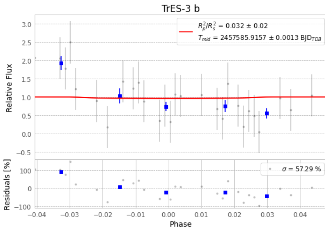
Figure 1 — FinalLightCurve_TrES-3 b_2016-07-16.png (SHA-256 0556cc4916903109...)
