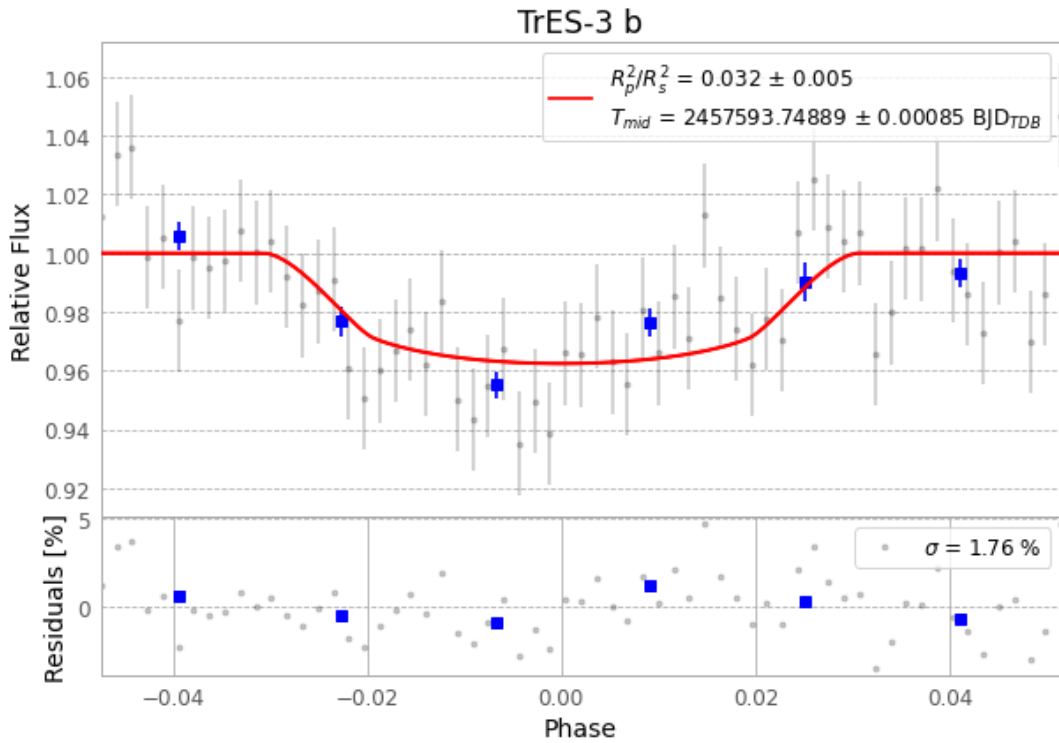
Figure 1 — FinalLightCurve_TrES-3 b_2016-07-23.png (SHA-256 39d577405a00203c...)
