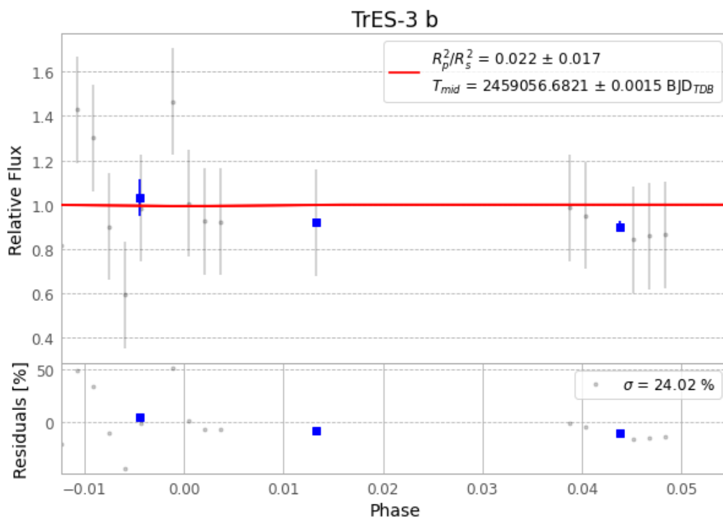
Figure 1 — FinalLightCurve_TrES-3 b_2020-07-25.png (SHA-256 d7ea2f473369e860...)
