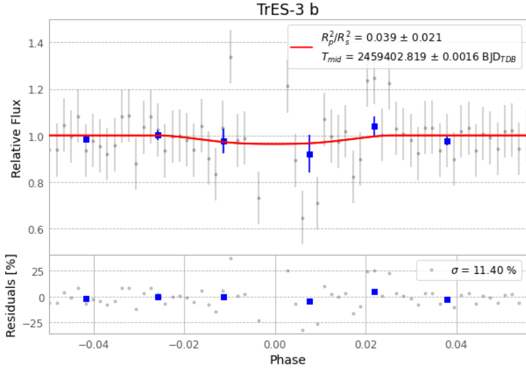
Figure 1 — FinalLightCurve_TrES-3 b_2021-07-06.png (SHA-256 42040186e5f7712e...)
