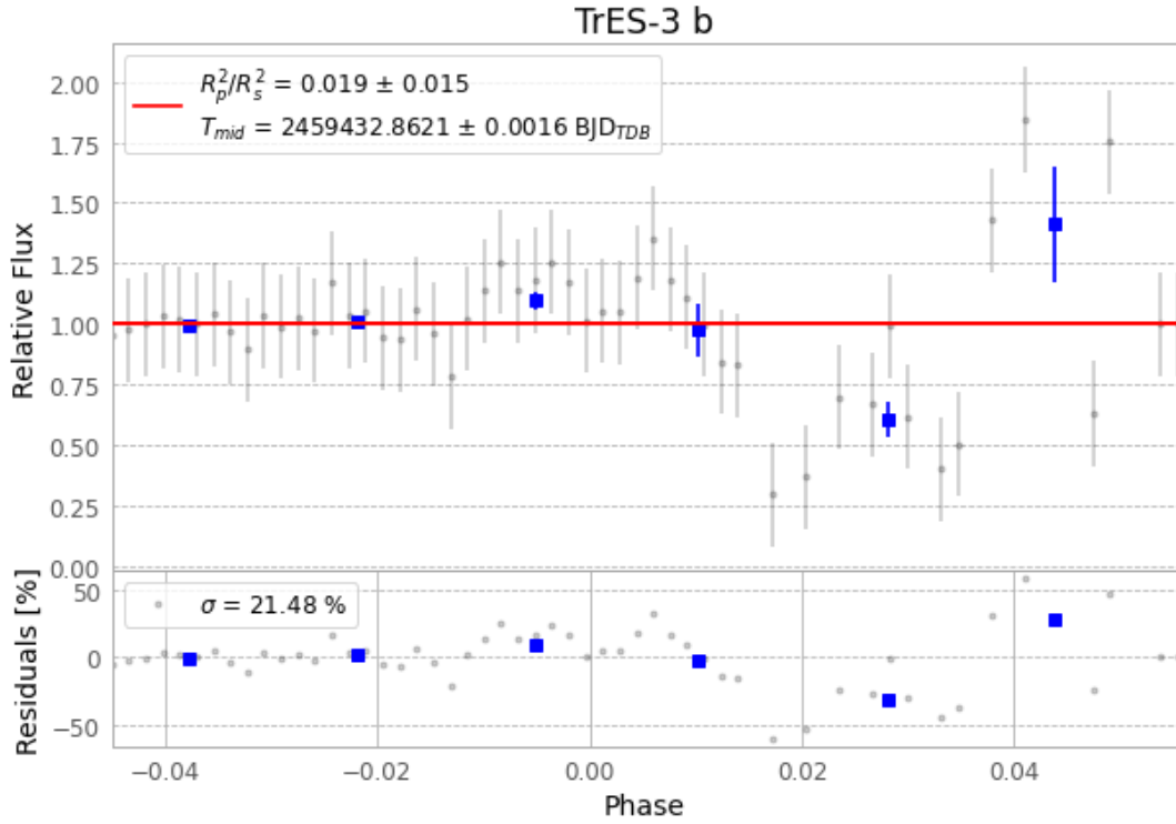
Figure 1 — FinalLightCurve_TrES-3 b_2021-08-06.png (SHA-256 c8c05b4c366a22c7...)
