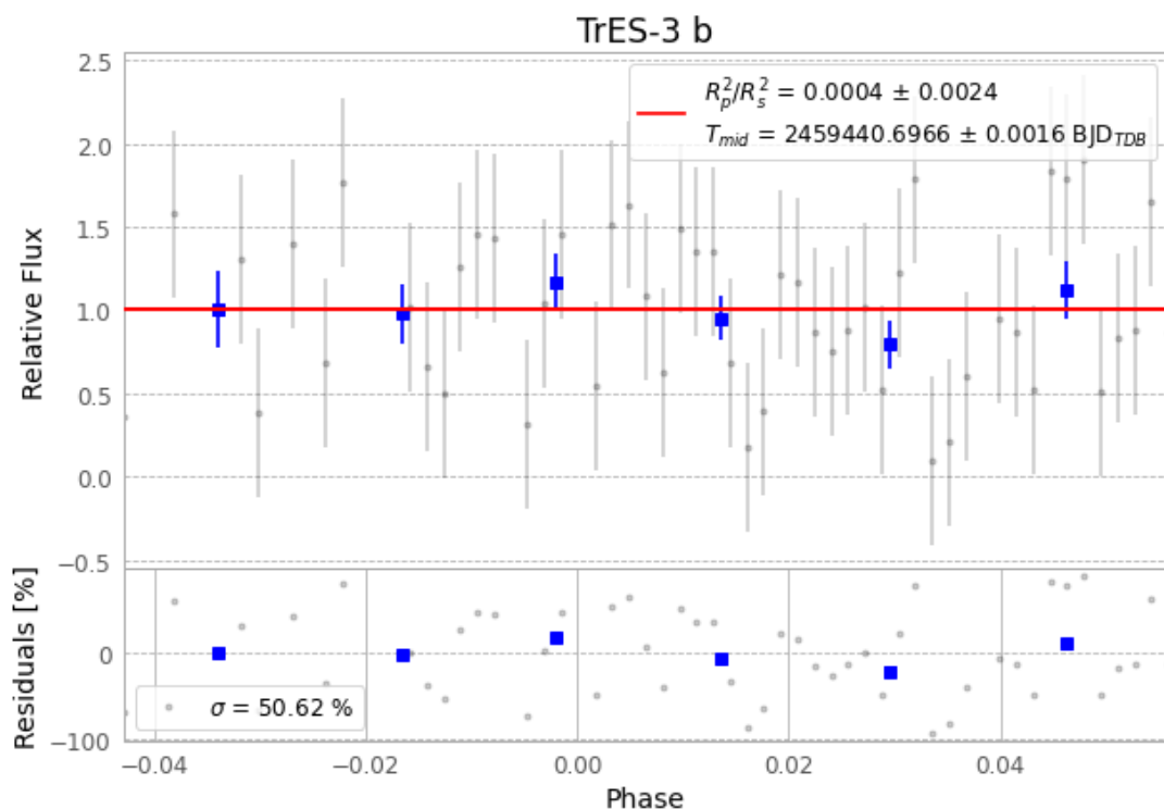
Figure 1 — FinalLightCurve_TrES-3 b_2021-08-13.png (SHA-256 dd1a53bf437dcd44...)
