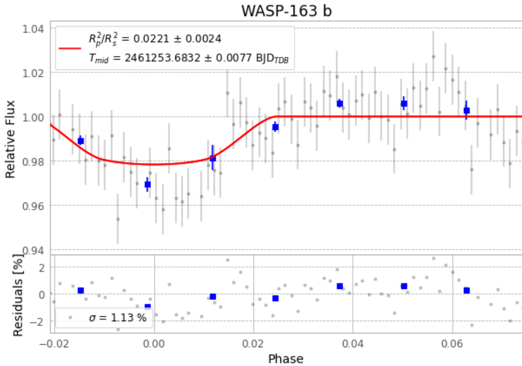
Figure 1 — FinalLightCurve_WASP-163 b_2026-07-31.png (SHA-256 d5485122cb5a8dcc...)
