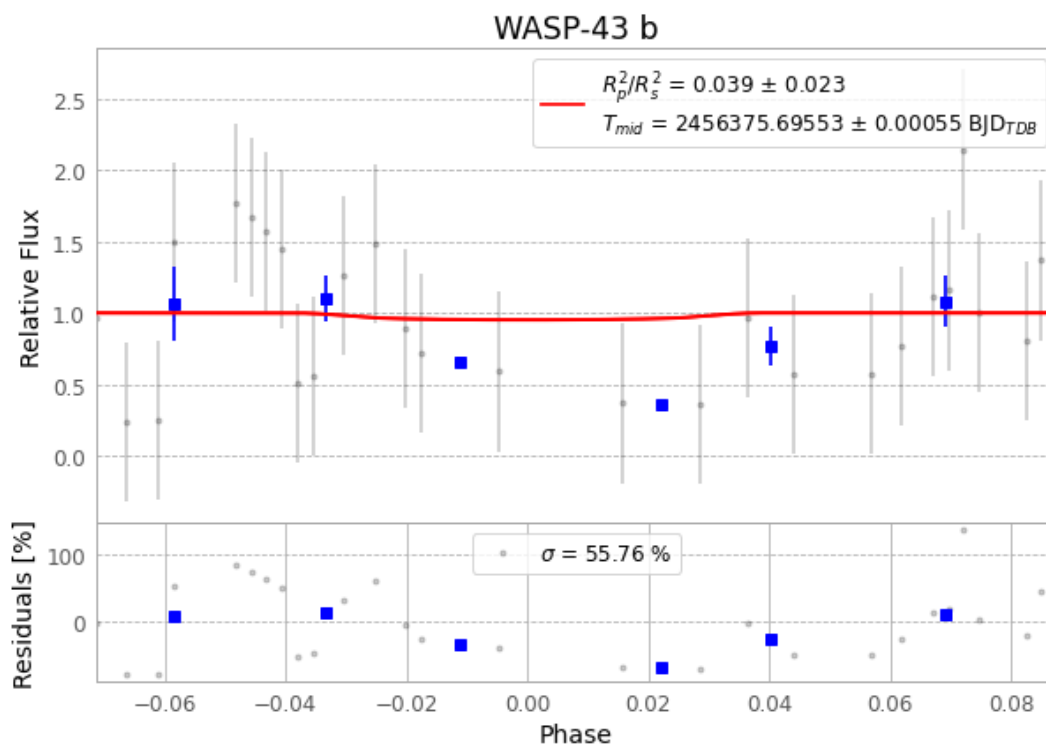
Figure 1 — FinalLightCurve_WASP-43 b_2013-03-23.png (SHA-256 c9346b074c4b2ef0...)
