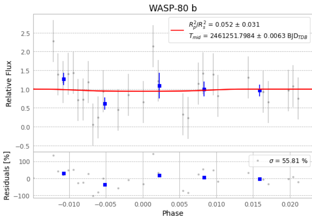
Figure 1 — FinalLightCurve_WASP-80 b_2026-07-29.png (SHA-256 04aa00302066871f...)
