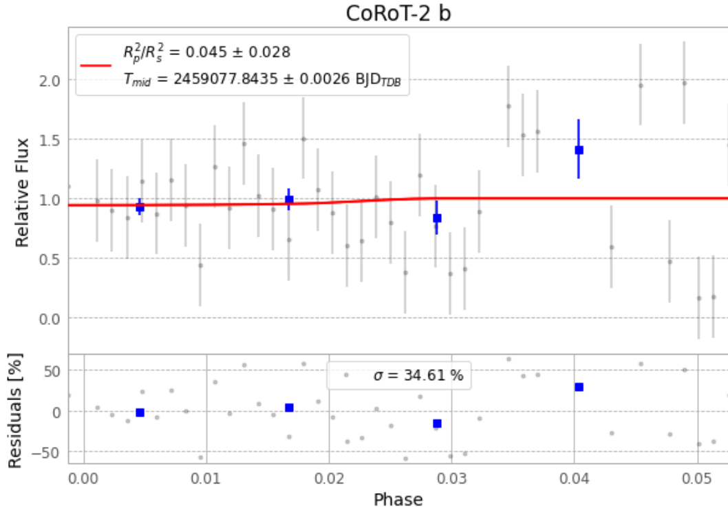
Figure 1 — FinalLightCurve_CoRoT-2 b_2020-08-16.png (SHA-256 c5390343bfa97609...)
